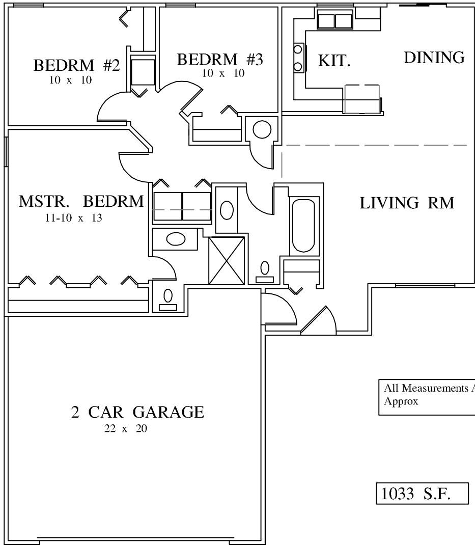
MAIN LEVEL FLR. PLAN 40 x 45-8
