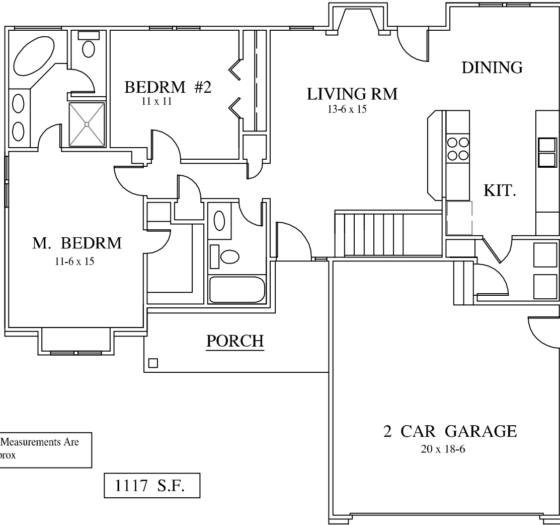
MAIN LEVEL FLR. PLAN 47-8 x 42-6
