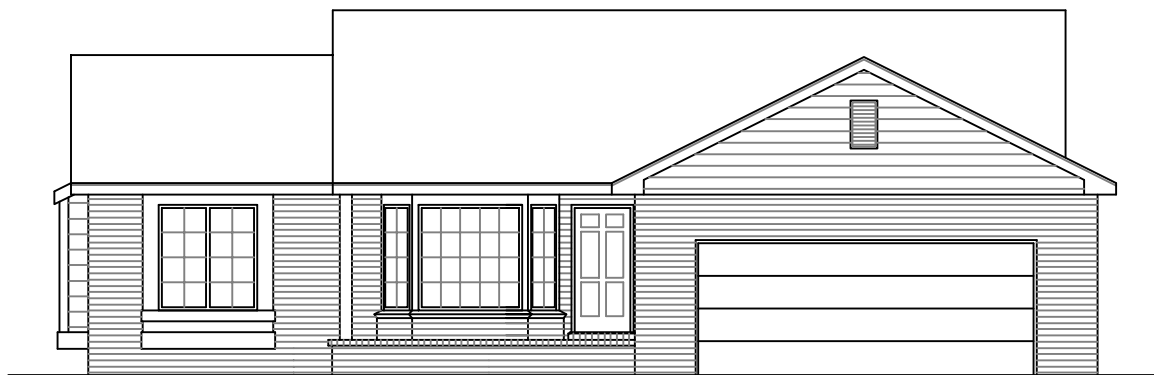
FRONT ELEVATION
