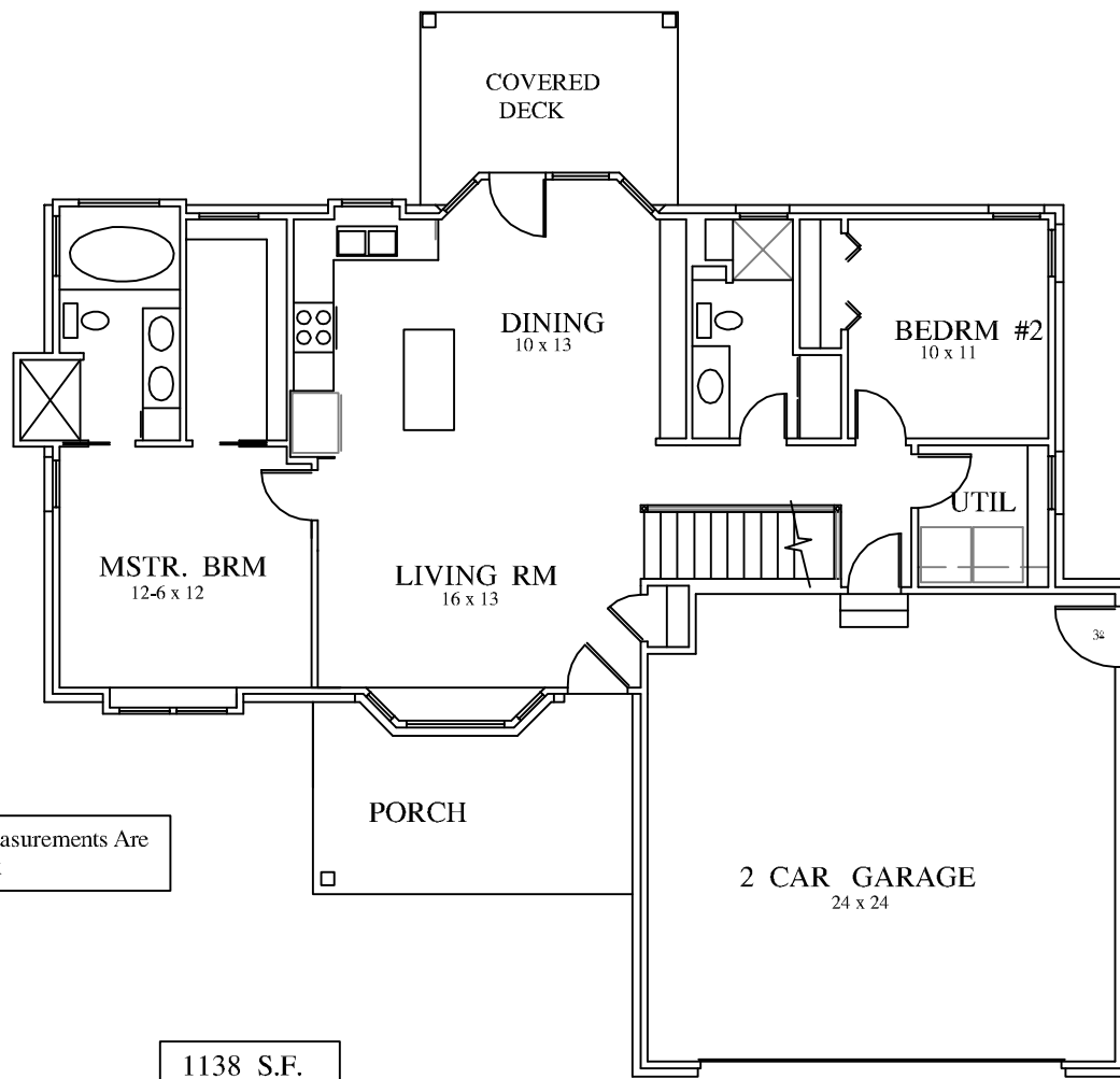
MAIN LEVEL FLR. PLAN 50-10 x 43-6
