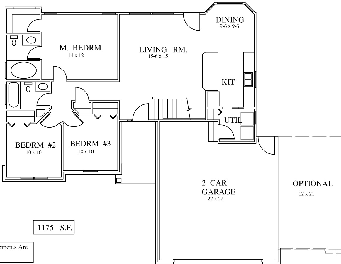
MAIN LEVEL FLR. PLAN 50 x 48
