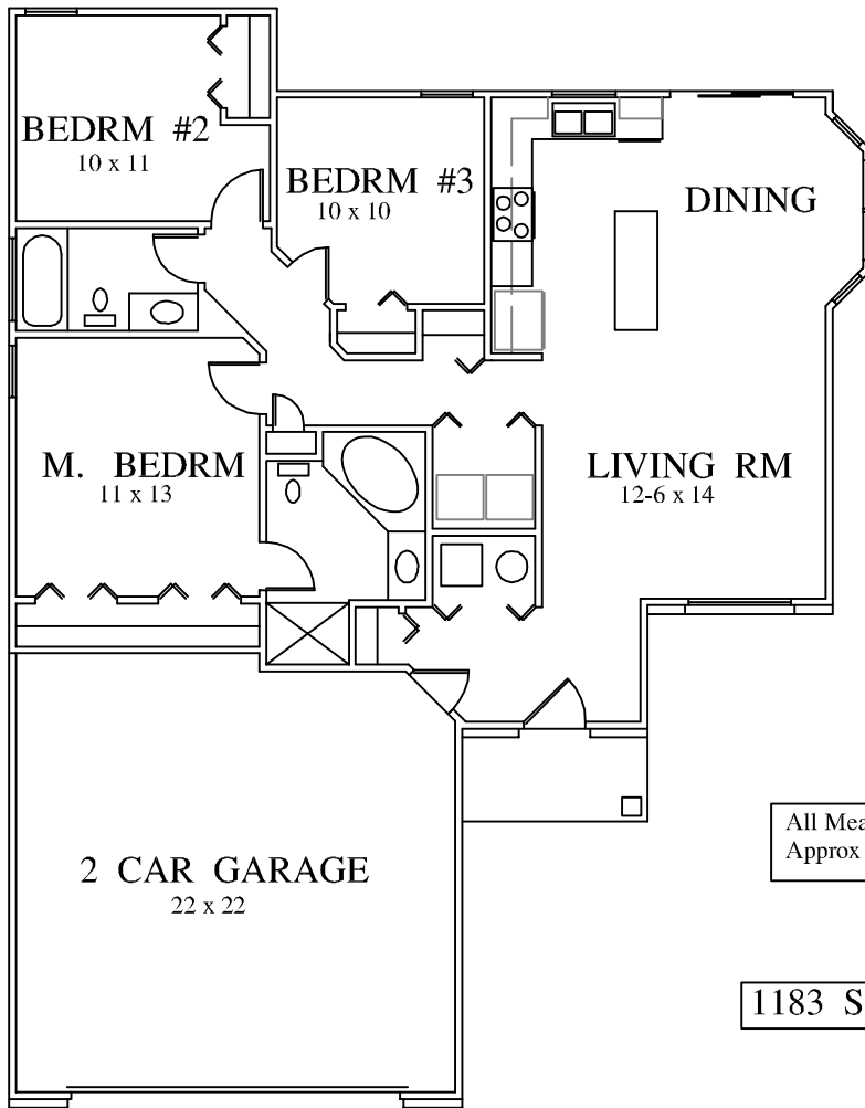
MAIN LEVEL FLR. PLAN 40 x 46
