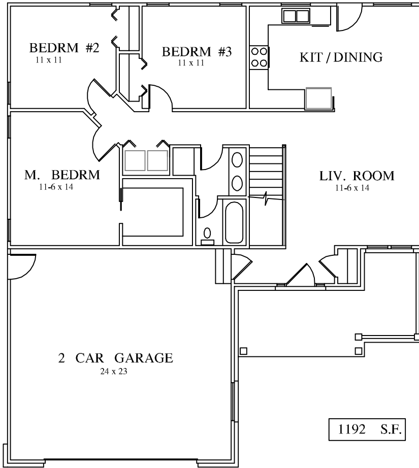
MAIN LEVEL FLR. PLAN 44 X 49
