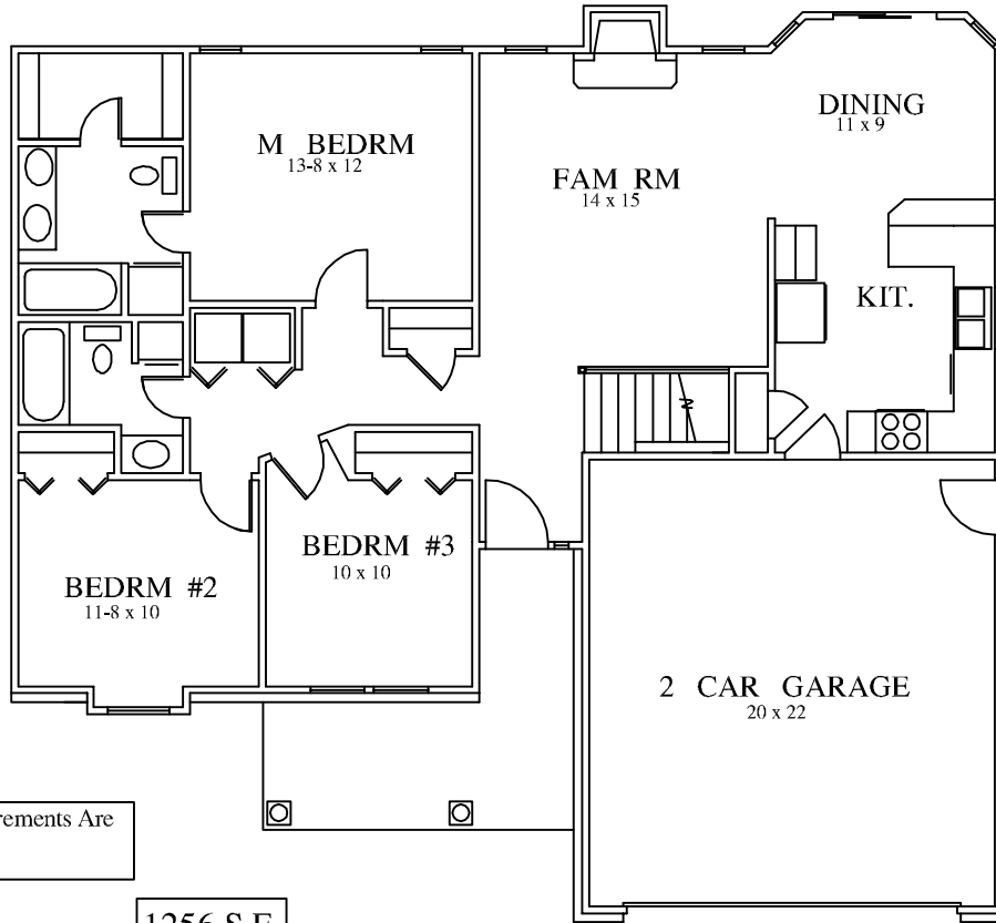
MAIN LEVEL FLOOR PLAN 42-5 x 48
