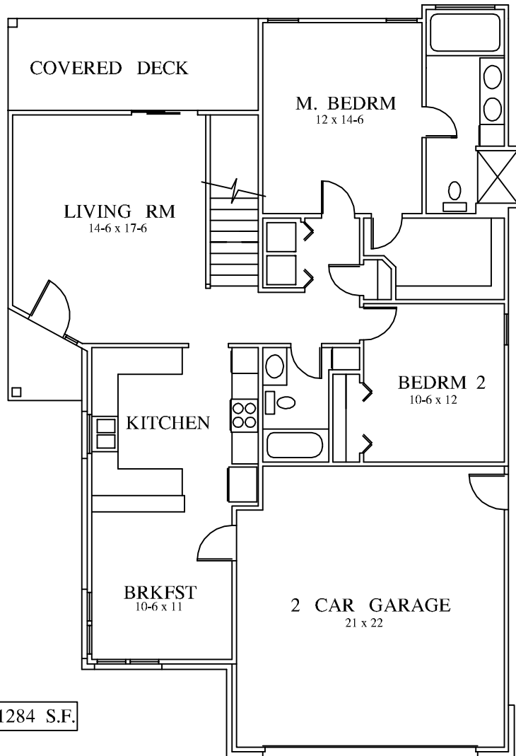
MAIN LEVEL FLR. PLAN 38 x 56
