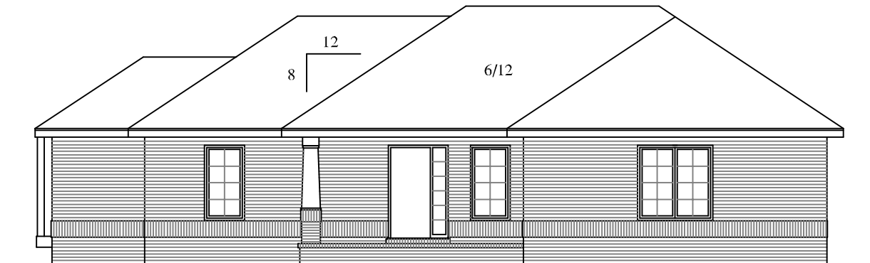
FRONT ELEVATION
