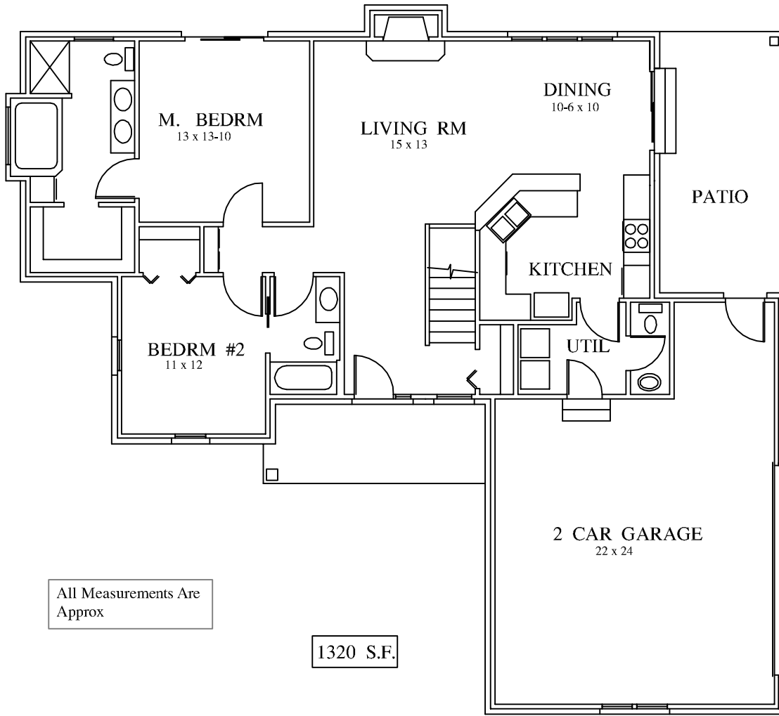
MAIN LEVEL FLR. PLAN 58-4 x 52
