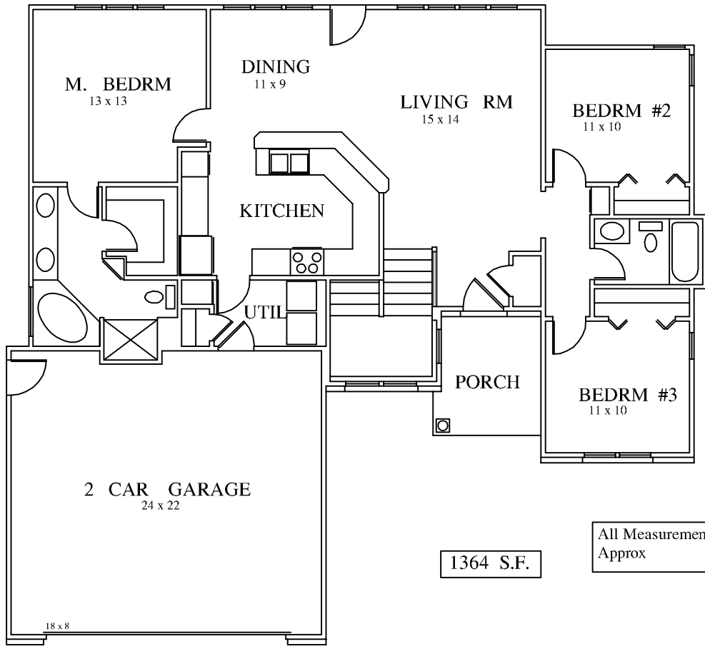
MAIN LEVEL FLR PLAN 52 x 48
